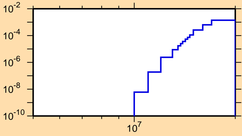
\sigma vs. E for ^{192}\text{Re}(n,d)
