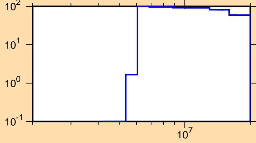
\Delta\sigma/\sigma vs. E for ^{193}\text{Re}(n,p)
