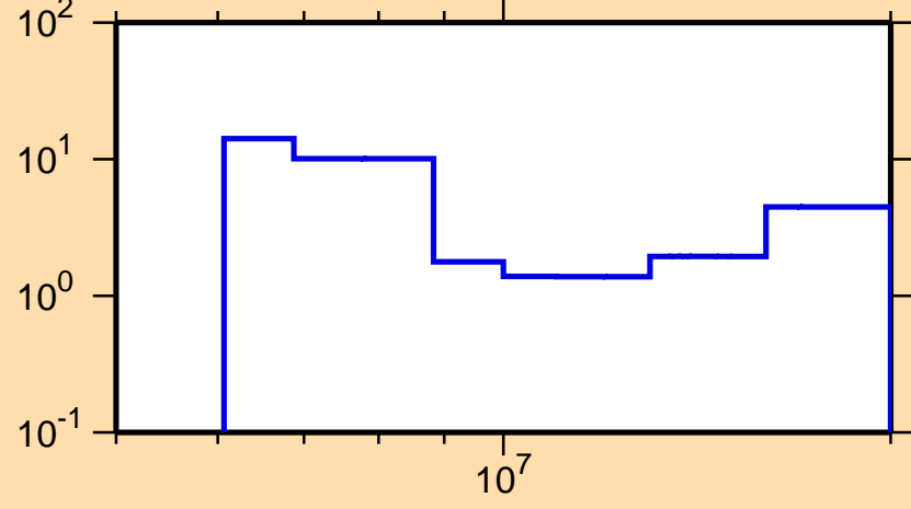
\Delta\sigma/\sigma vs. E for ^{193}\text{Re}(n,\text{tot.})
