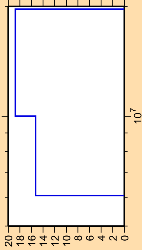
\Delta\sigma/\sigma vs. E for ^{193}\text{Re}(n,2n)
