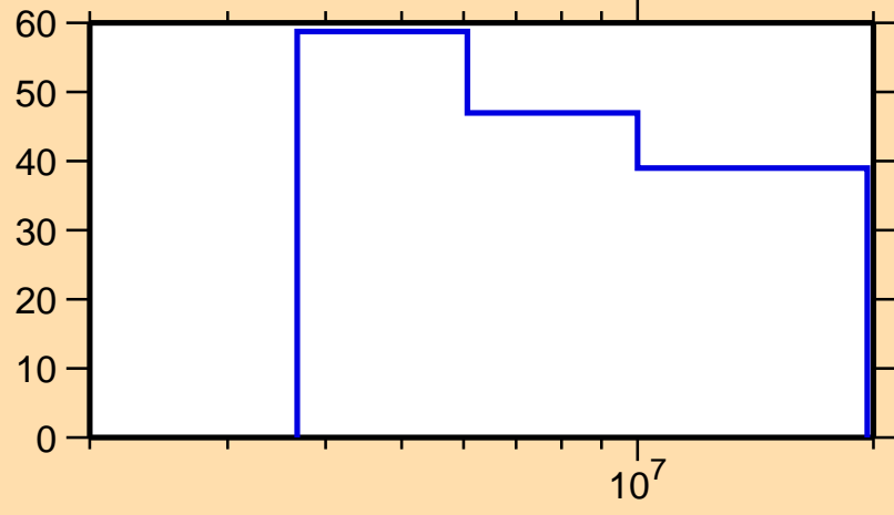
\Delta\sigma/\sigma vs. E for ^{193}\text{Re}(n,n_1)
