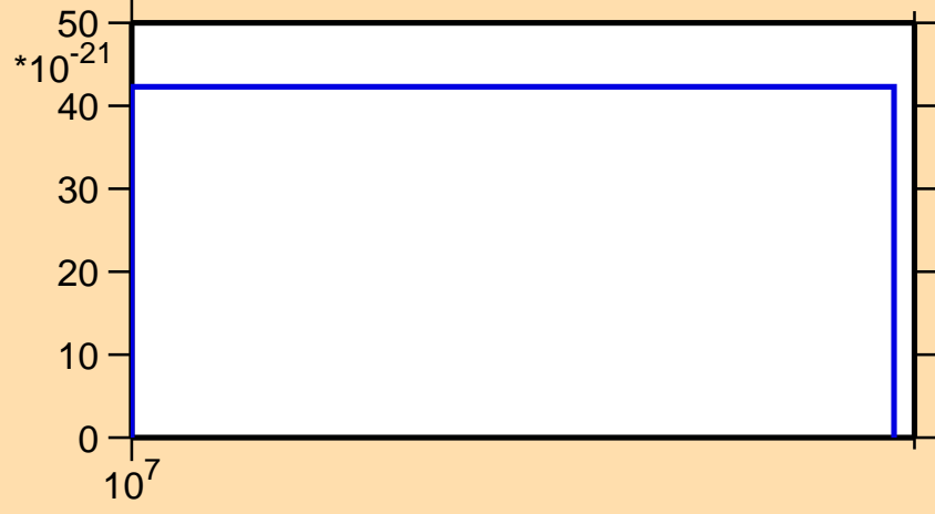
\sigma vs. E for ^{193}\text{Re}(\text{mt } 42)
