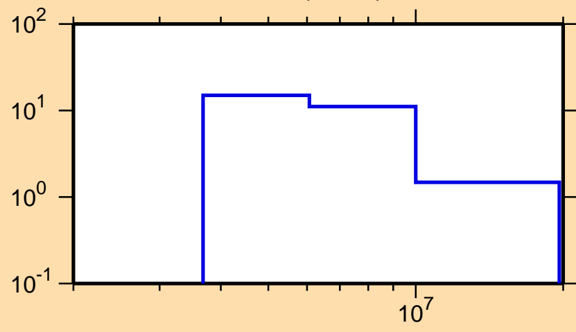
\Delta\sigma/\sigma vs. E for ^{193}\text{Re}(n,\text{tot.})
