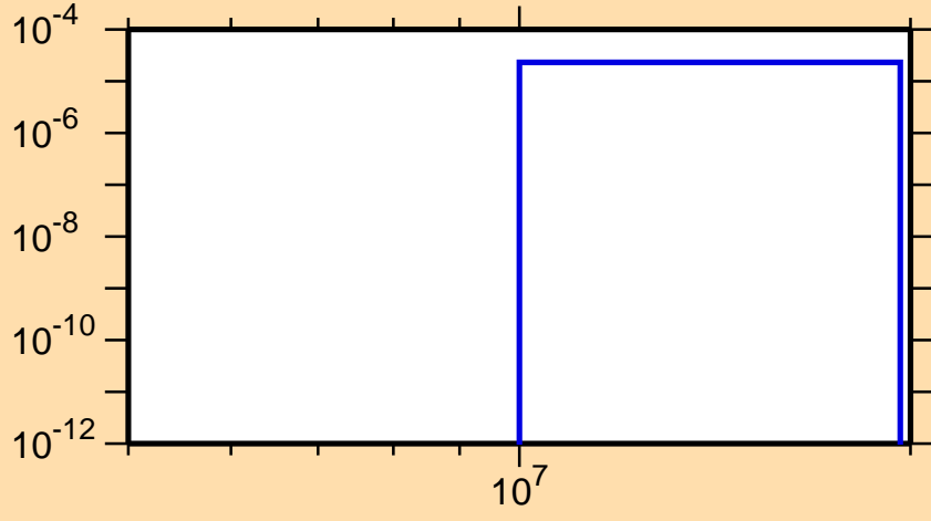
\sigma vs. E for ^{193}\text{Re}(n,np)
