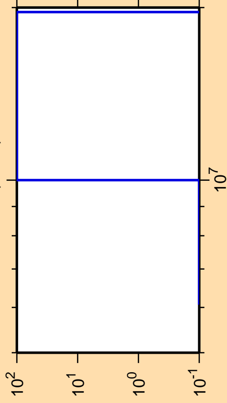
\Delta\sigma/\sigma vs. E for ^{193}\text{Re}(n,\alpha)
