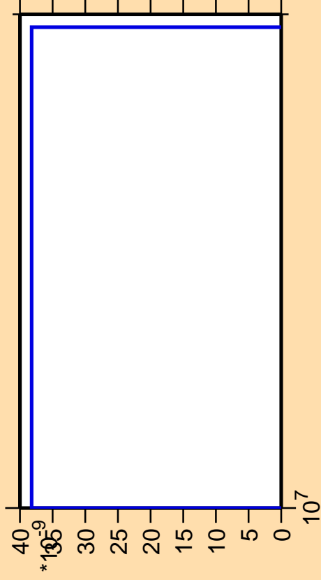
\Delta\sigma/\sigma vs. E for ^{193}\text{Re}(\text{mt } 42)
