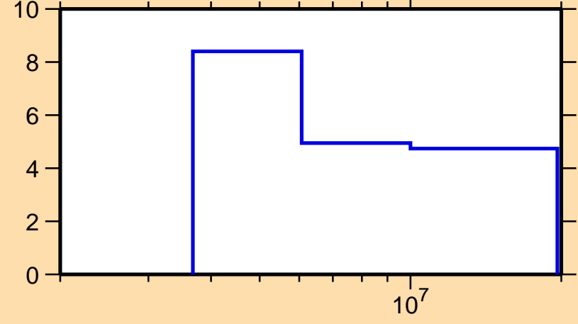
\Delta\sigma/\sigma vs. E for ^{193}\text{Re}(n,\text{nonel.})
