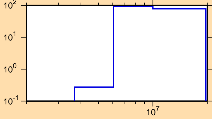
\Delta\sigma/\sigma vs. E for ^{193}\text{Re}(n,p)
