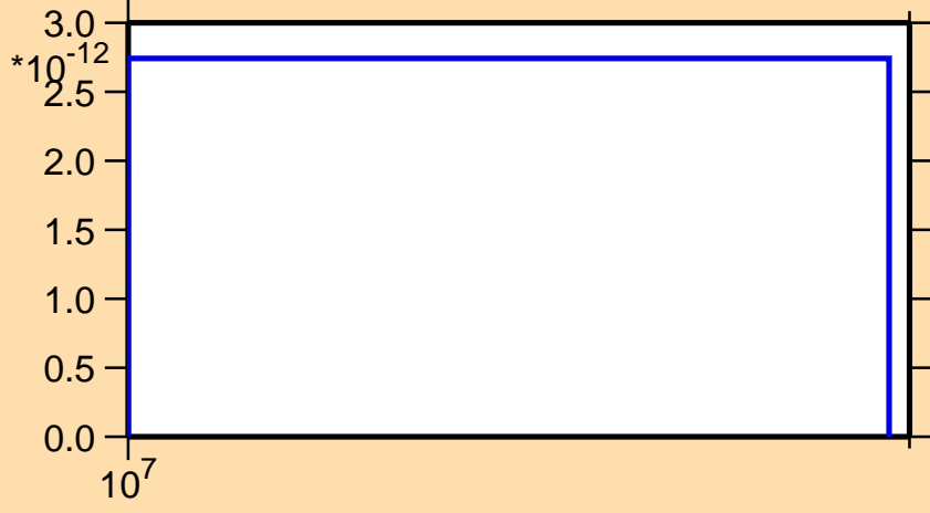
\sigma vs. E for ^{193}\text{Re}(n,2n\alpha)
