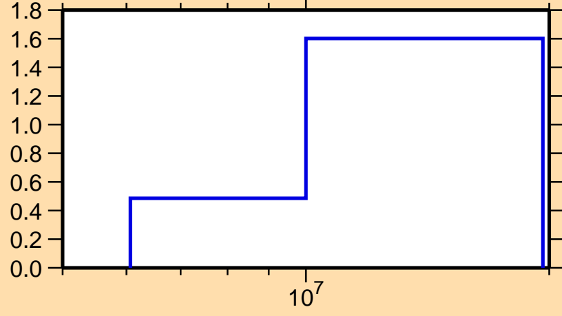
\sigma vs. E for ^{193}\text{Re}(n,2n)
