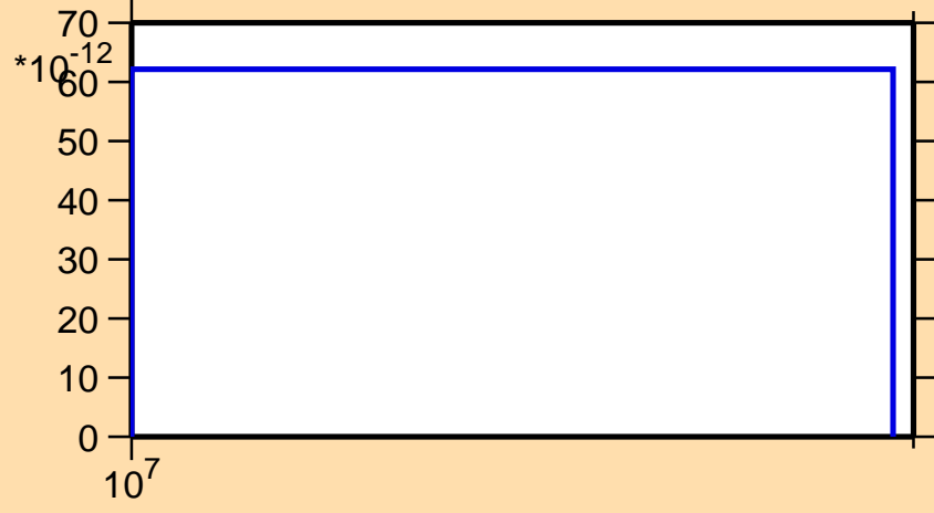
\sigma vs. E for ^{193}\text{Re}(n,2np)
