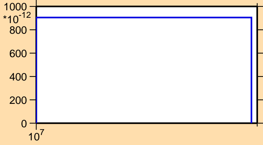
\sigma vs. E for ^{193}\text{Re}(n,\text{nd})
