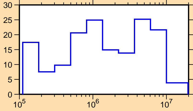
\Delta\sigma/\sigma vs. E for ^{193}\text{Re}(n, el.)
