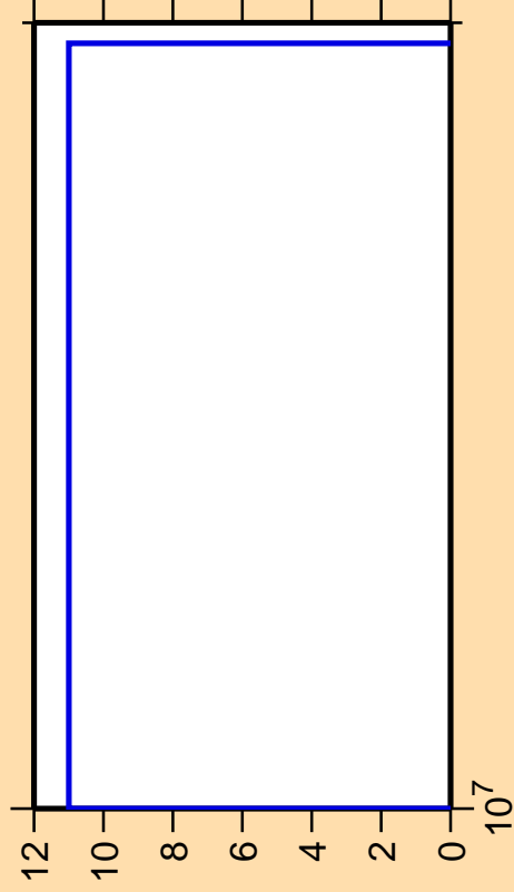
\Delta\sigma/\sigma vs. E for ^{193}\text{Re}(n,3n)
