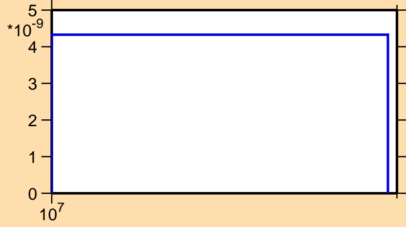
\sigma vs. E for ^{193}\text{Re}(n,nt)
