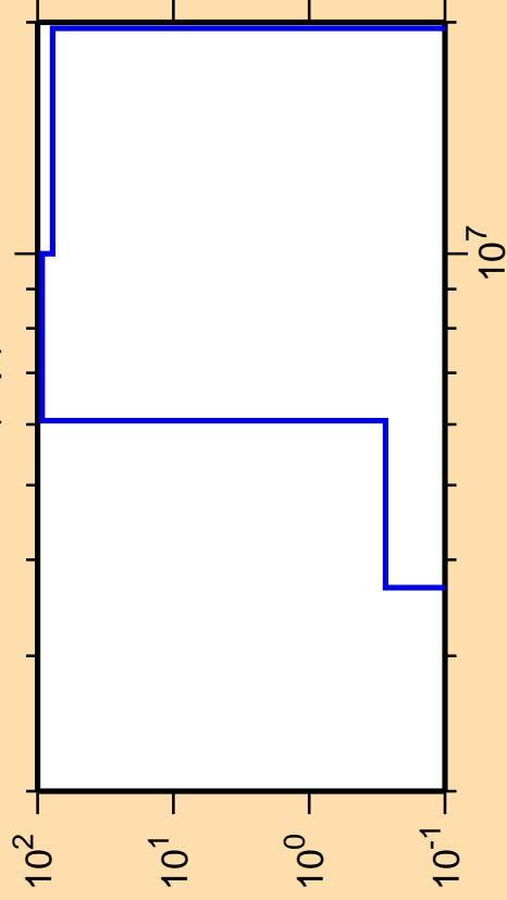
\Delta\sigma/\sigma vs. E for ^{193}\text{Re}(n,p)
