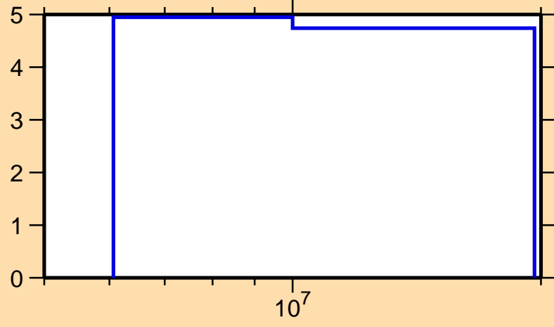
\Delta\sigma/\sigma vs. E for ^{193}\text{Re}(n,\text{nonel.})
