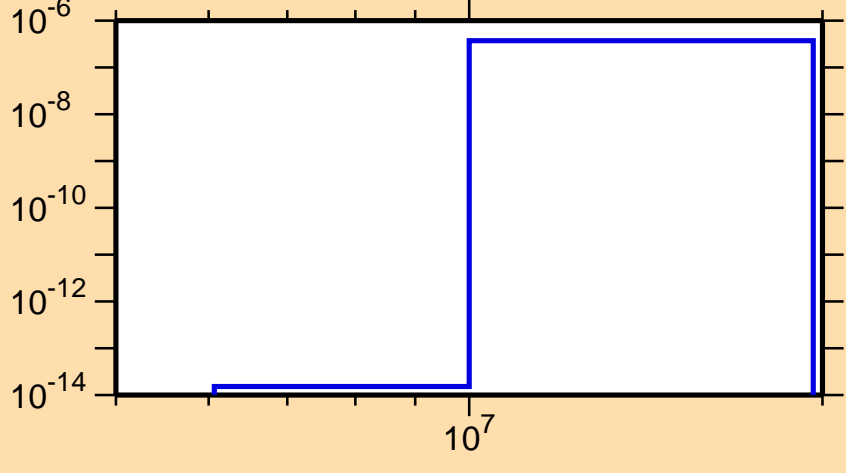
\sigma vs. E for ^{193}\text{Re}(n,\alpha)
