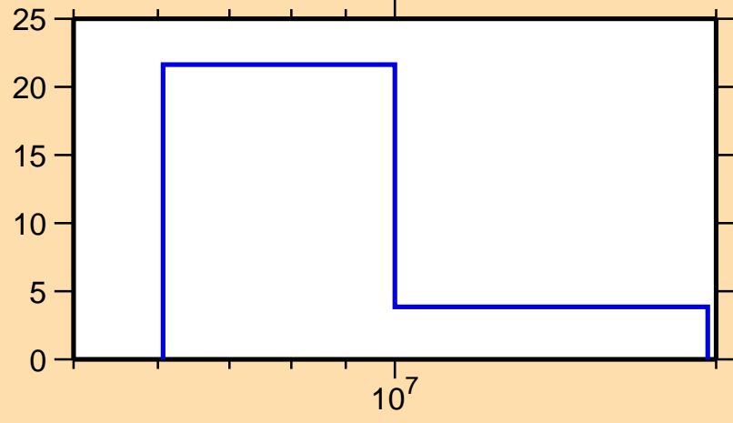
\Delta\sigma/\sigma vs. E for ^{193}\text{Re}(n,\text{el.})
