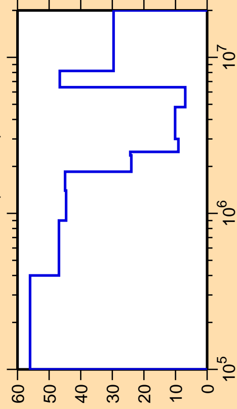
\Delta\sigma/\sigma vs. E for ^{193}\text{Re}(n,\text{inel.})
