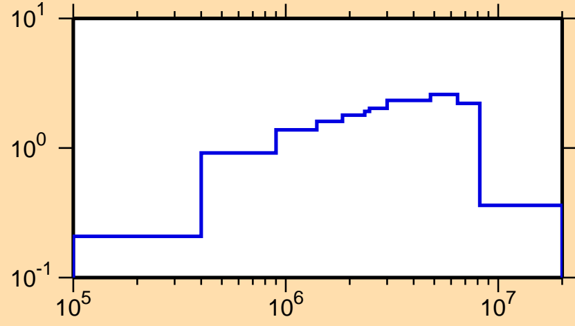
\sigma vs. E for ^{193}\text{Re}(n,\text{inel.})
