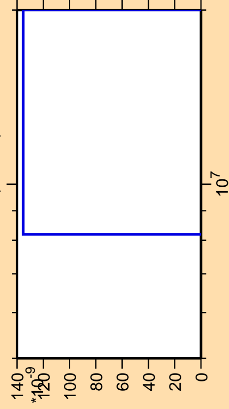
\Delta\sigma/\sigma vs. E for ^{193}\text{Re}(\text{mt } 42)
