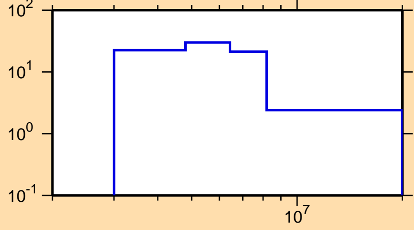
\Delta\sigma/\sigma vs. E for ^{193}\text{Re}(n,\text{el.})
