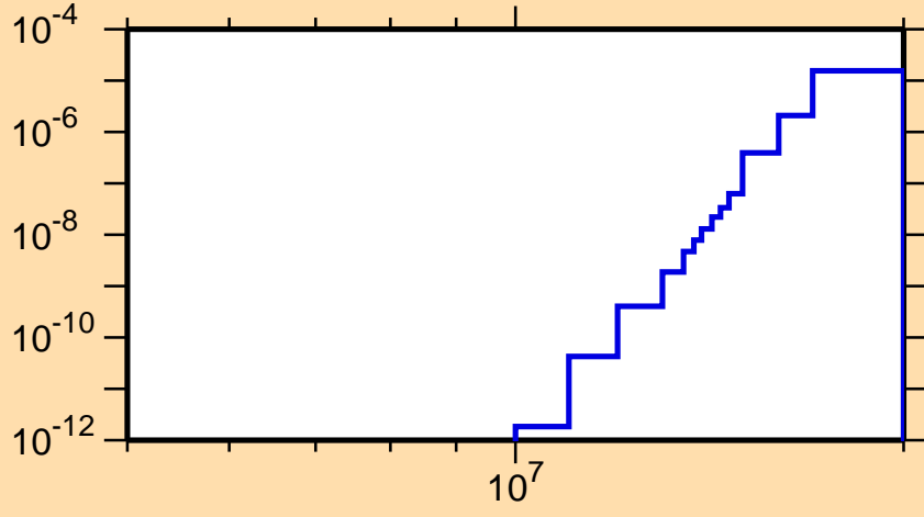
\sigma vs. E for ^{194}\text{Re}(n,\alpha)
