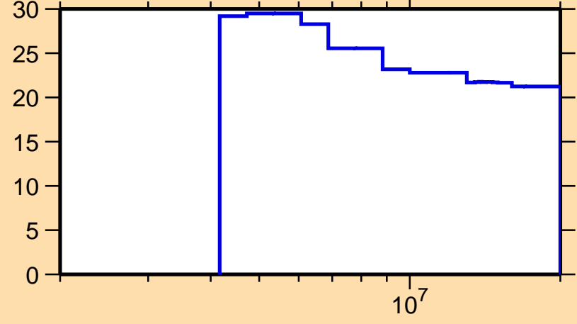
\Delta\sigma/\sigma vs. E for ^{194}\text{Re}(n,\text{nonel.})
