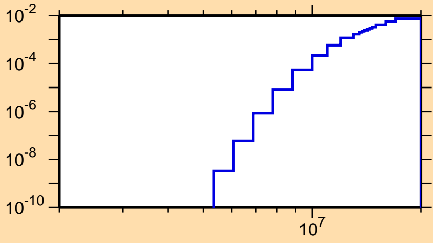
\sigma vs. E for ^{194}\text{Re}(n,p)
