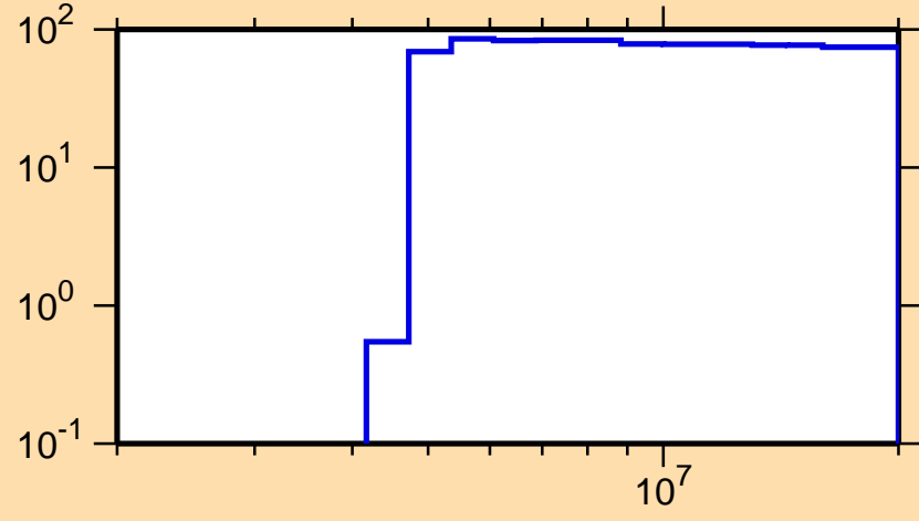
\Delta\sigma/\sigma vs. E for ^{194}\text{Re}(n,p)
