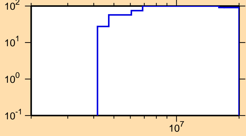
\Delta\sigma/\sigma vs. E for ^{194}\text{Re}(n,n\text{cont.})
