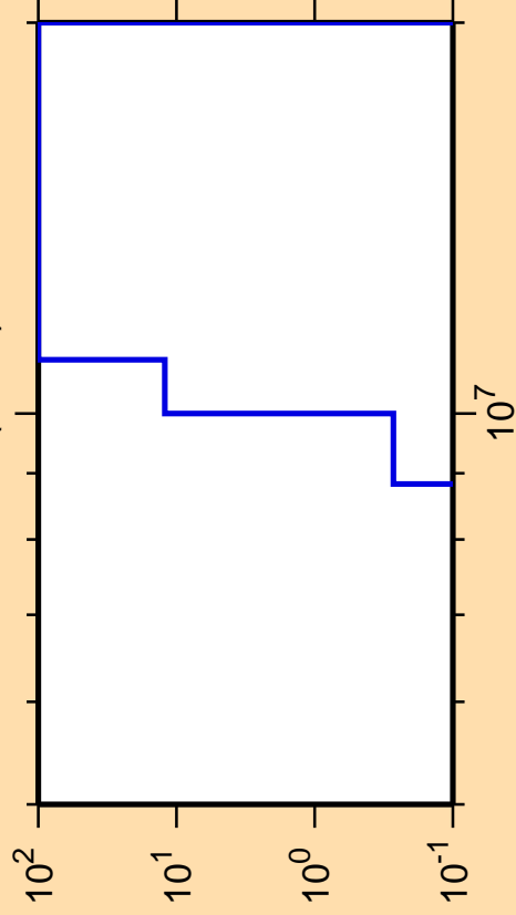
\Delta\sigma/\sigma vs. E for ^{194}\text{Re}(n,\alpha)
