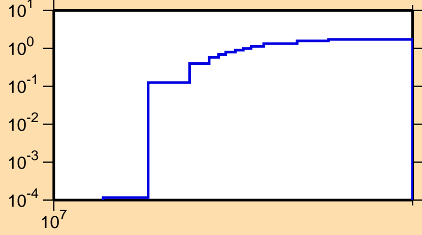
\sigma vs. E for ^{194}\text{Re}(n,3n)
