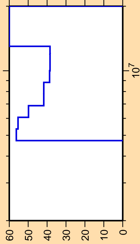
\Delta\sigma/\sigma vs. E for ^{194}\text{Re}(n,2n)
