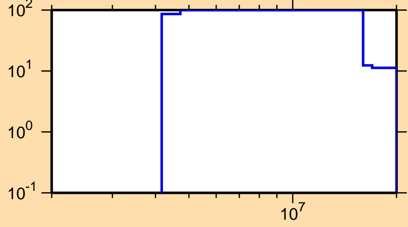
\Delta\sigma/\sigma vs. E for ^{194}\text{Re}(n,n_1)
