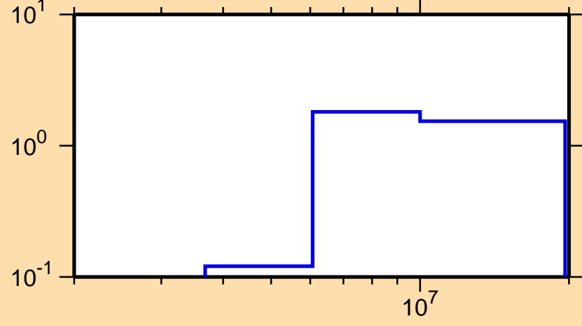
\sigma vs. E for ^{194}\text{Re}(n,2n)
