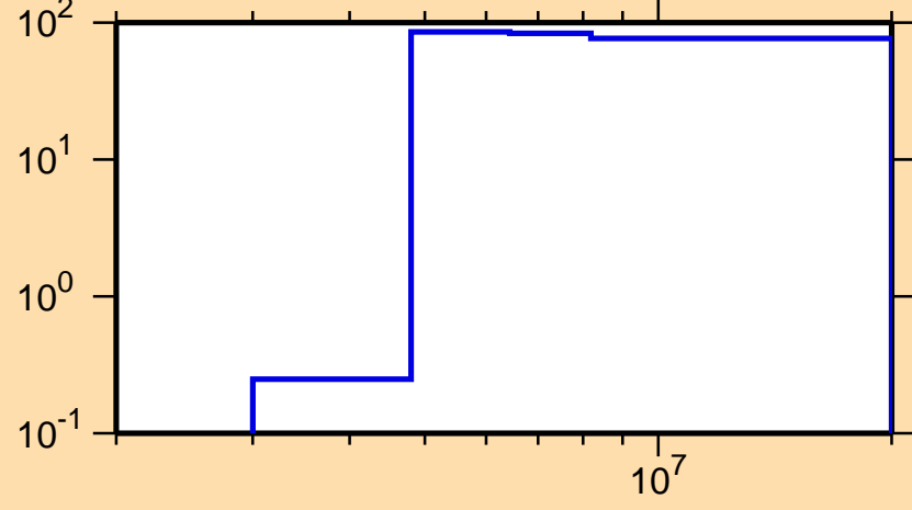
\Delta\sigma/\sigma vs. E for ^{194}\text{Re}(n,p)
