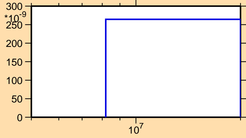
\sigma vs. E for ^{194}\text{Re}(n,\alpha)
