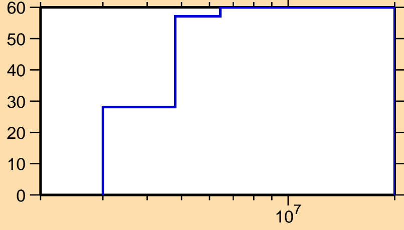
\Delta\sigma/\sigma vs. E for ^{194}\text{Re}(n,n\text{cont.})
