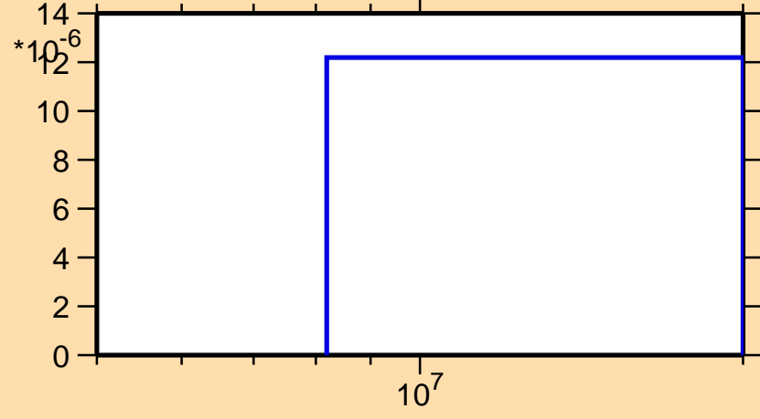
\sigma vs. E for ^{194}\text{Re}(n,t)
