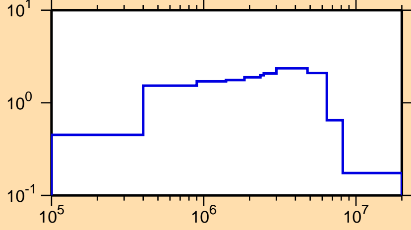
\sigma vs. E for ^{194}\text{Re}(n,\text{inel.})
