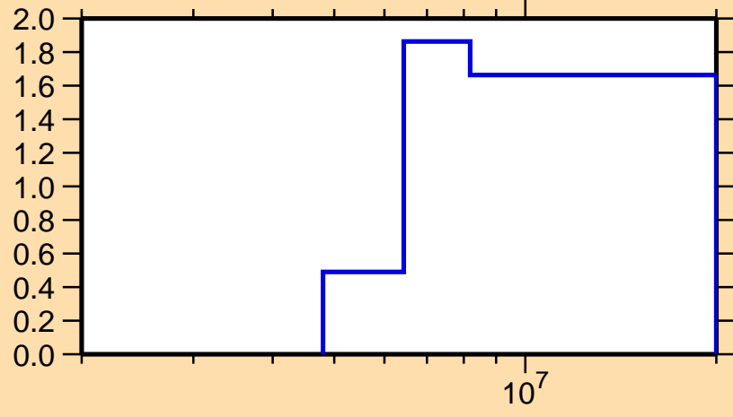
\sigma vs. E for ^{194}\text{Re}(n,2n)
