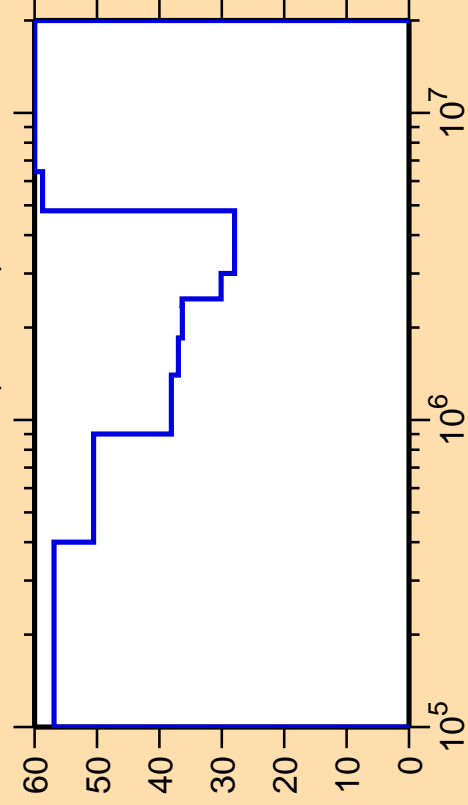
\Delta\sigma/\sigma vs. E for ^{194}\text{Re}(n,\text{inel.})
