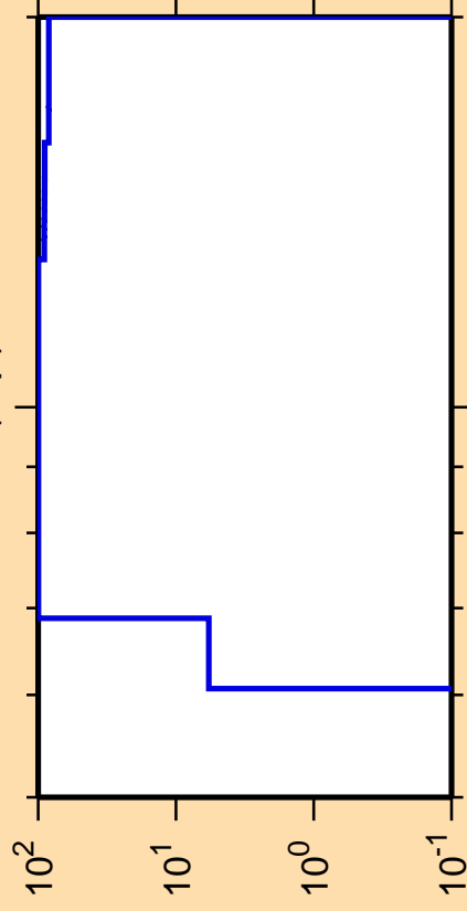
\Delta\sigma/\sigma vs. E for ^{195}\text{Re}(n,p)
