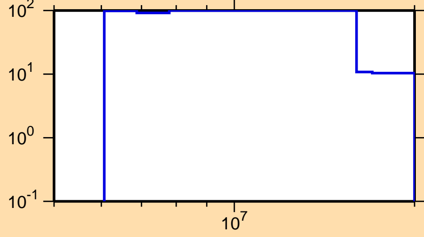
\Delta\sigma/\sigma vs. E for ^{195}\text{Re}(n,n_1)
