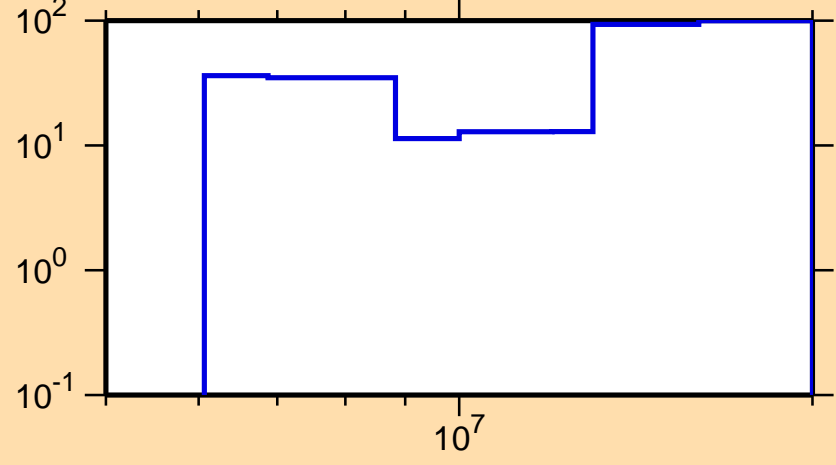
\Delta\sigma/\sigma vs. E for ^{195}\text{Re}(n,2n)
