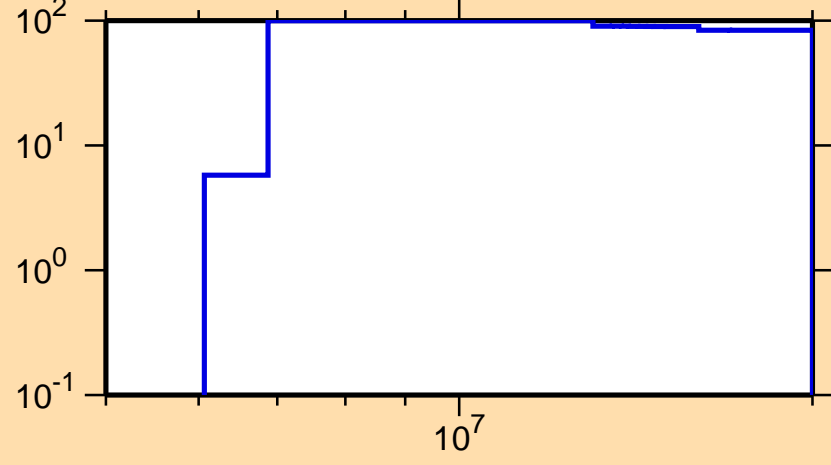
\Delta\sigma/\sigma vs. E for ^{195}\text{Re}(n,p)
