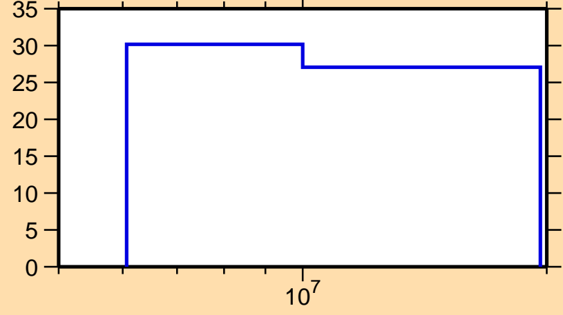
\Delta\sigma/\sigma vs. E for ^{195}\text{Re}(n,el.)
