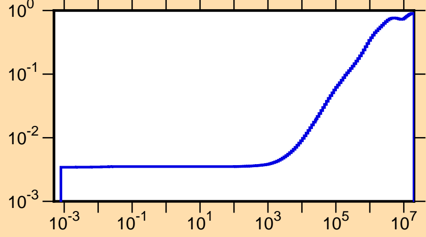
\mu vs. E for ^{196}\text{Re}(\text{mt251})
