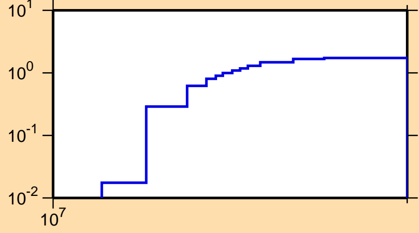
\sigma vs. E for ^{196}\text{Re}(n,3n)
