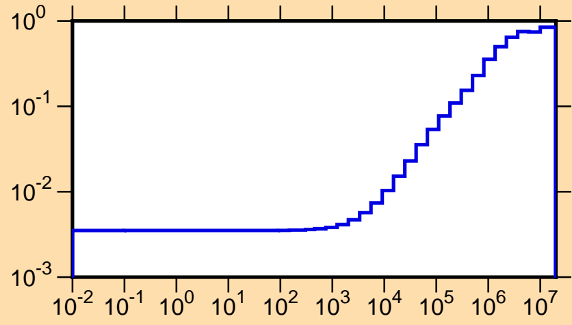
\mu vs. E for ^{196}\text{Re}(\text{mt251})
