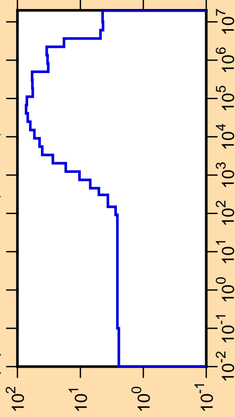
\Delta\mu/\mu vs. E for ^{196}\text{Re}(\text{mt251})
