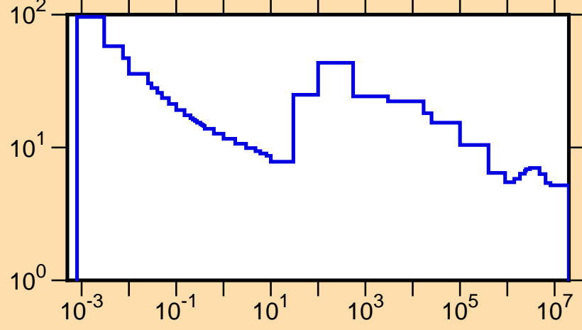
\sigma vs. E for ^{196}\text{Re}(n,\text{tot.})
