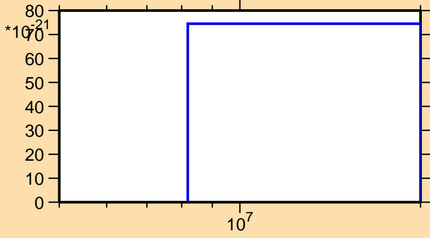
\sigma vs. E for ^{196}\text{Re}(\text{mt } 42)
