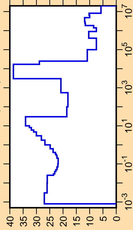
\Delta\sigma/\sigma vs. E for ^{196}\text{Re}(n,\text{tot.})
