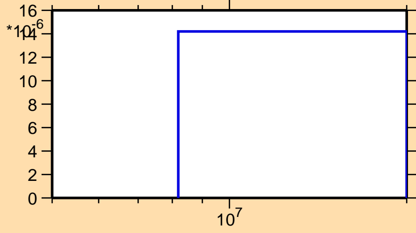
\sigma vs. E for ^{196}\text{Re}(n,d)
