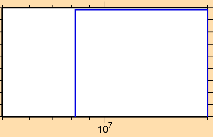
\sigma vs. E for ^{255}
