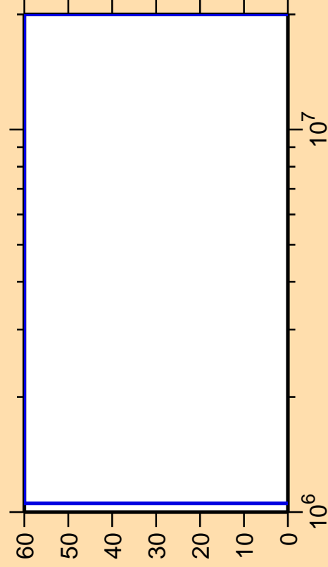
\Delta\sigma/\sigma vs. E for ^{257}\text{Pu}
