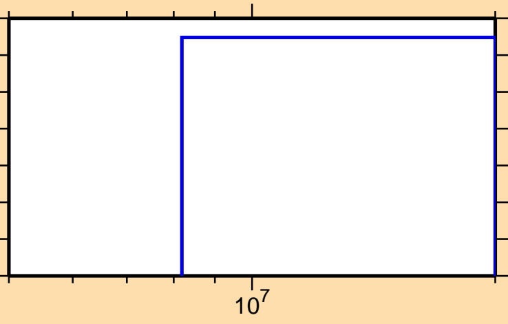
\sigma vs. E for ^{257}
