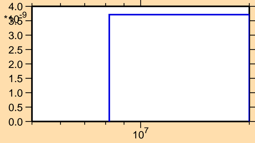
\sigma vs. E for ^{257}\text{He3} )
