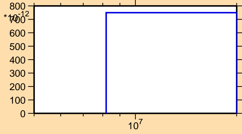
\sigma vs. E for ^{259}\text{He3} )
