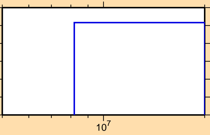
\sigma vs. E for ^{259}
