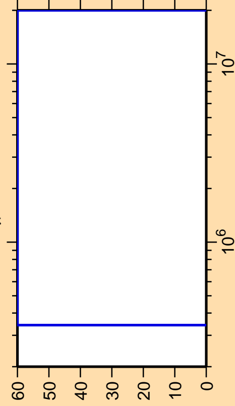
\Delta\sigma/\sigma vs. E for ^{261}\gamma
