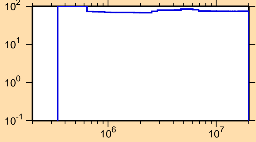
\Delta\sigma/\sigma vs. E for ^{261}
