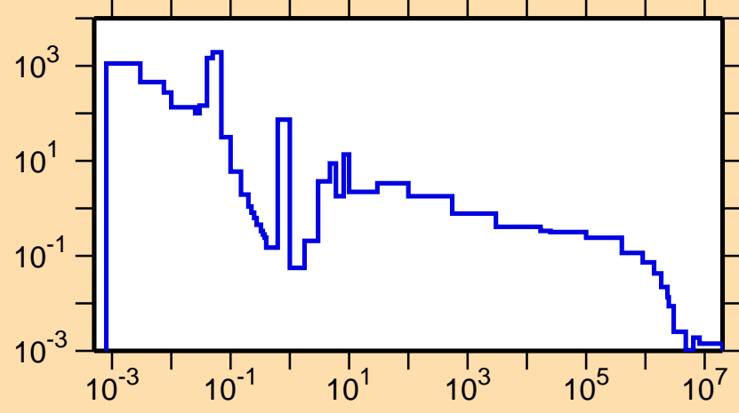
\sigma vs. E for ^{261}\text{Gd}
