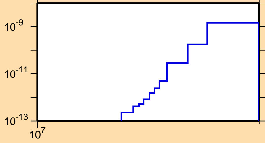
\sigma vs. E for ^{263}\text{He3} )
