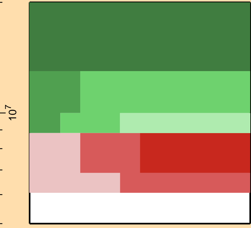
Correlation Matrix
