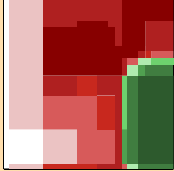
\Delta\sigma/\sigma vs. E for ^{263}
