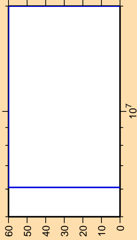
\Delta\sigma/\sigma vs. E for ^{264}\gamma
