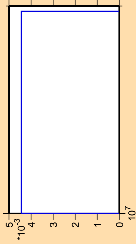
\Delta\sigma/\sigma vs. E for ^{264}\alpha )
