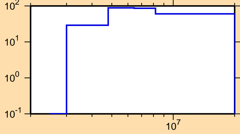
\Delta\sigma/\sigma vs. E for ^{264}
