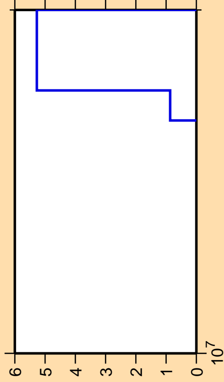
\Delta\sigma/\sigma vs. E for ^{266}\alpha )
