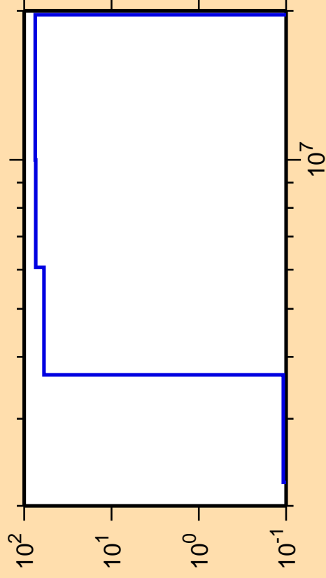
\Delta\sigma/\sigma vs. E for ^{267}\text{Gd}
