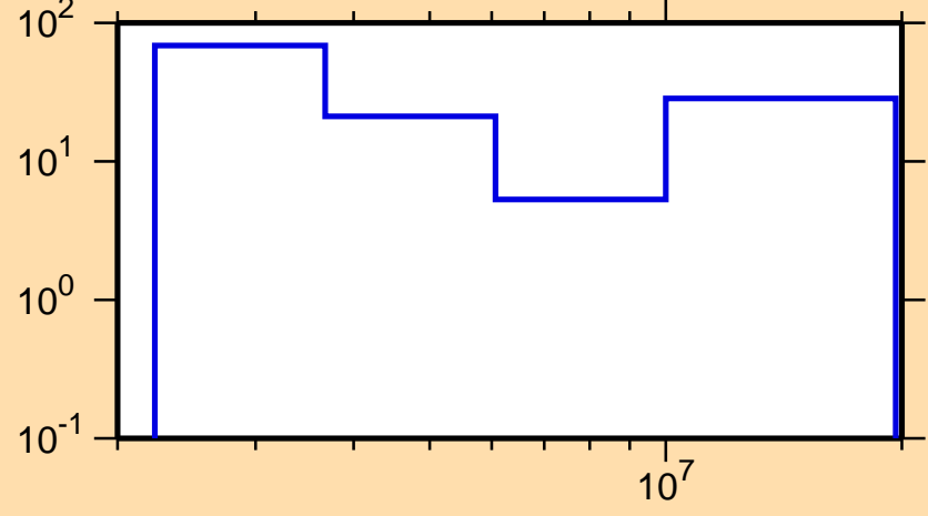
\Delta\sigma/\sigma vs. E for ^{267}\text{Gd}
