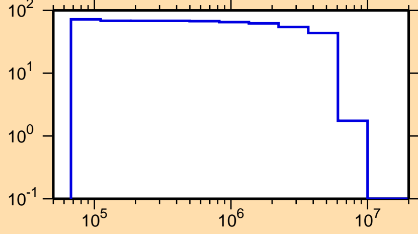
\Delta\sigma/\sigma vs. E for ^{280}_1
