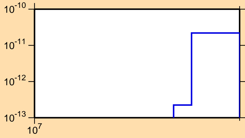
\sigma vs. E for ^{281}\text{He3} )
