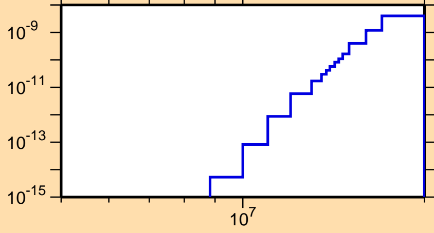
\sigma vs. E for ^{282}\text{He3} )
