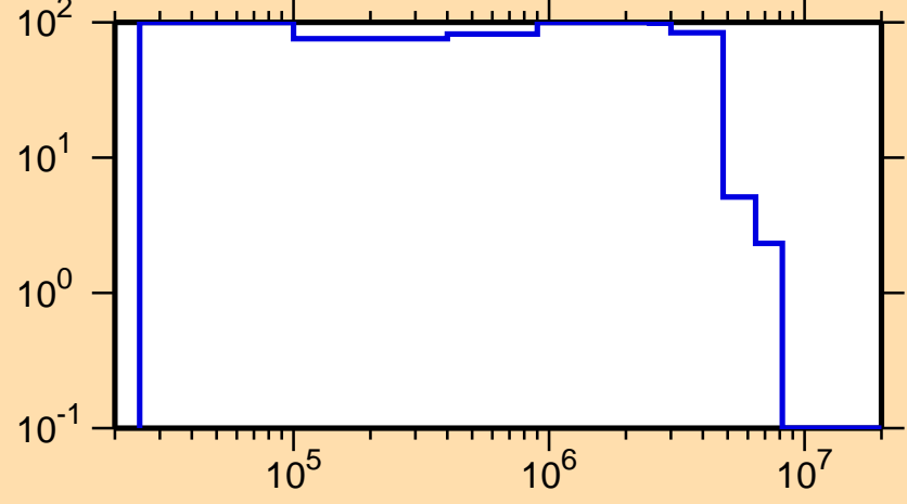
\Delta\sigma/\sigma vs. E for ^{282}_1
