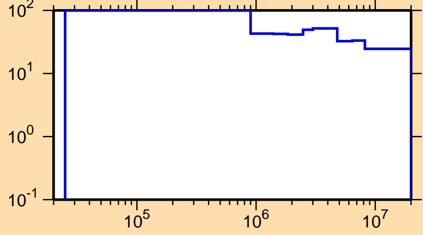
\Delta\sigma/\sigma vs. E for ^{282}
