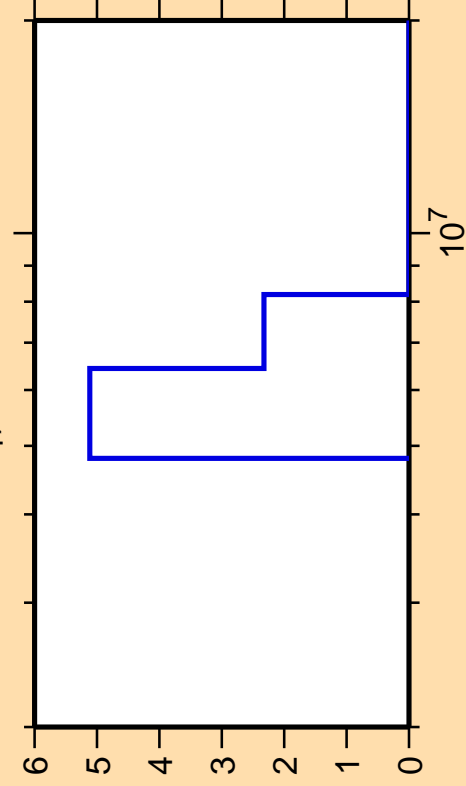
\Delta\sigma/\sigma vs. E for ^{282}\text{Po}
