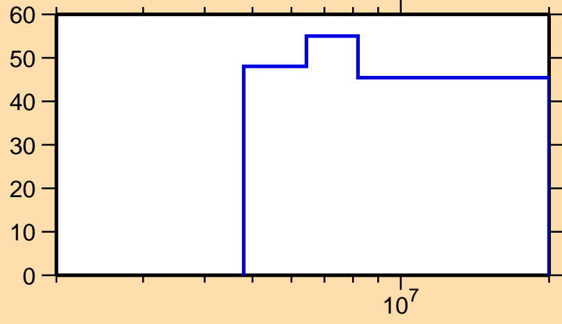
\Delta\sigma/\sigma vs. E for ^{282}\text{Po}
