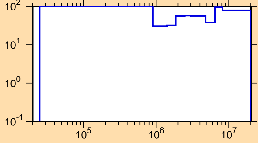
\Delta\sigma/\sigma vs. E for ^{283}
