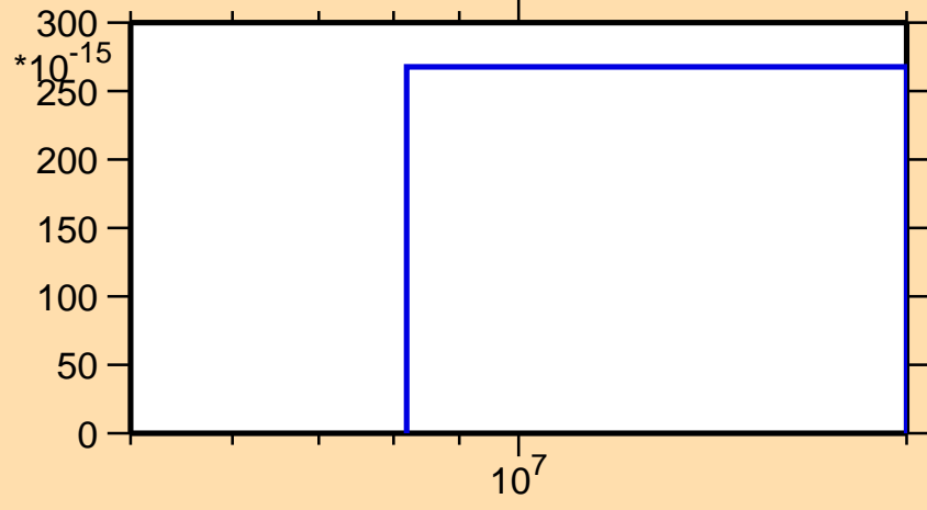
\sigma vs. E for ^{91}\text{Rh} (mt 34)
