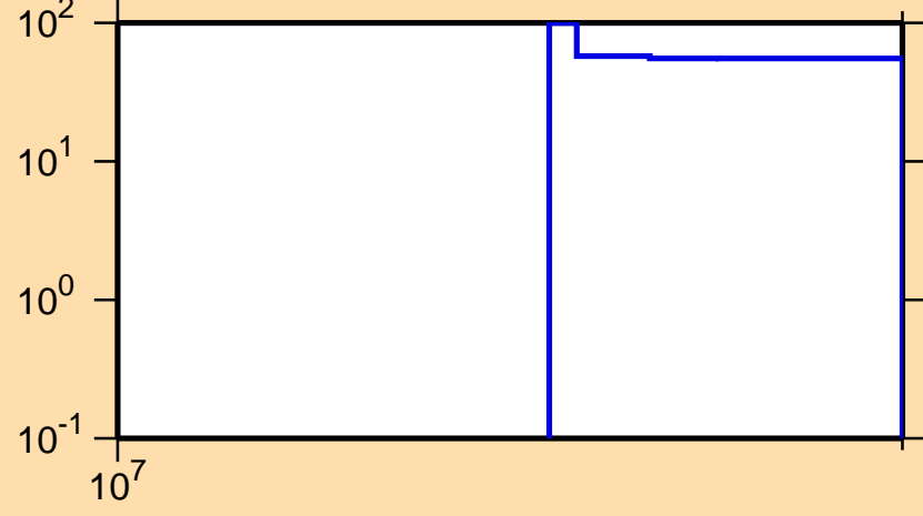
\Delta\sigma/\sigma vs. E for ^{91}\text{Rh}(n,2n)
