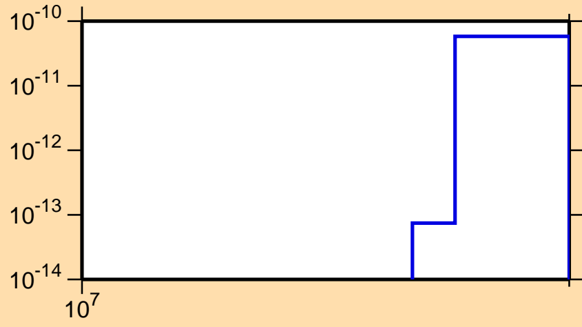
\sigma vs. E for ^{91}\text{Rh} (mt 34)
