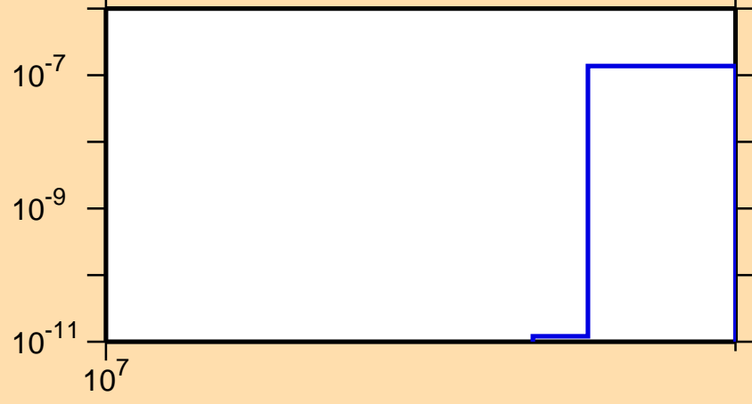
\sigma vs. E for ^{93}\text{Rh}(n,\text{pt})
