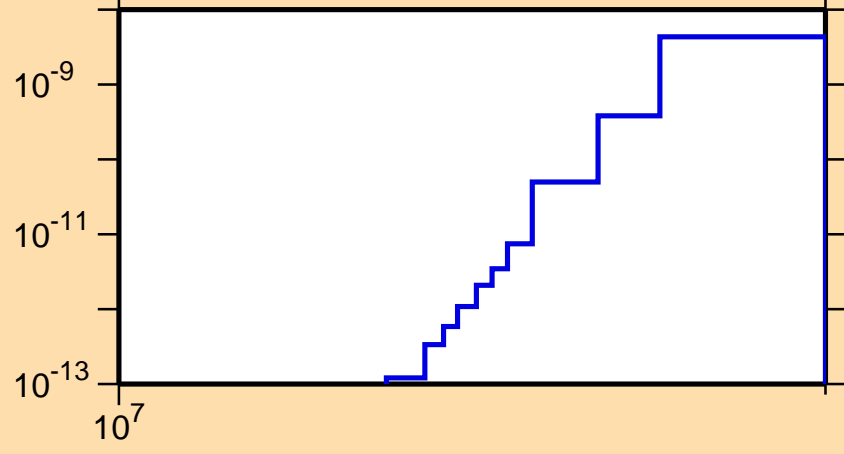
\sigma vs. E for ^{93}\text{Rh}(\text{mt117})
