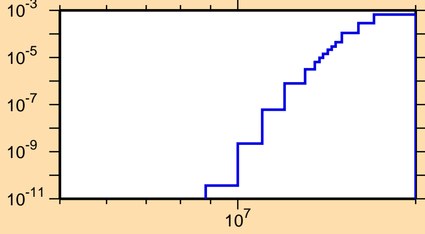
\sigma vs. E for ^{93}\text{Rh}(n,\alpha)
