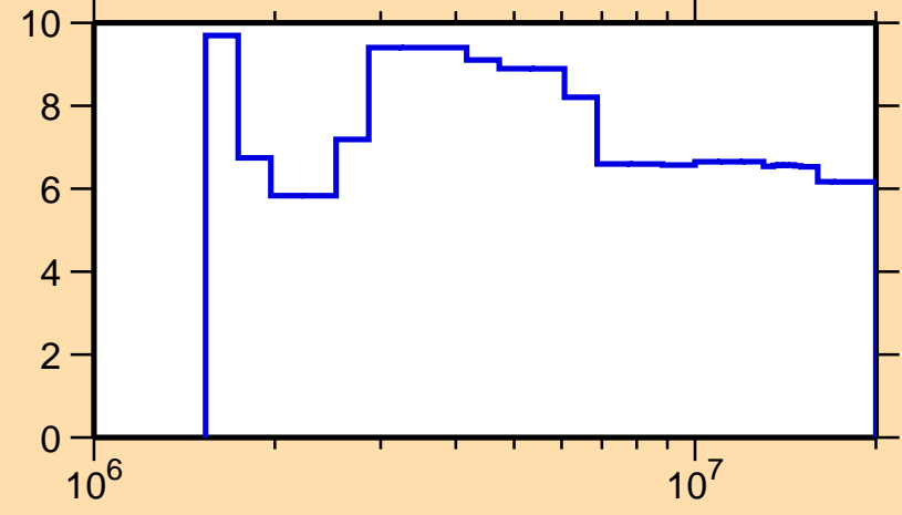
\Delta\sigma/\sigma vs. E for ^{93}\text{Rh}(n,n\text{onel.})
