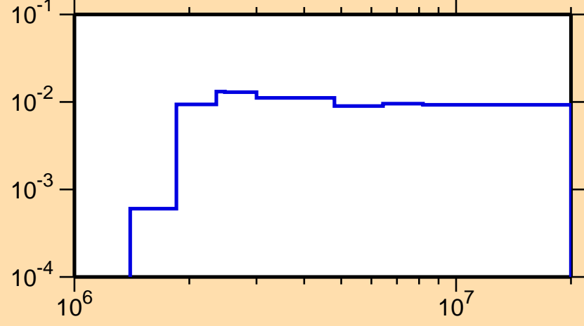
\sigma vs. E for ^{93}\text{Rh}(n,n\text{cont.})
