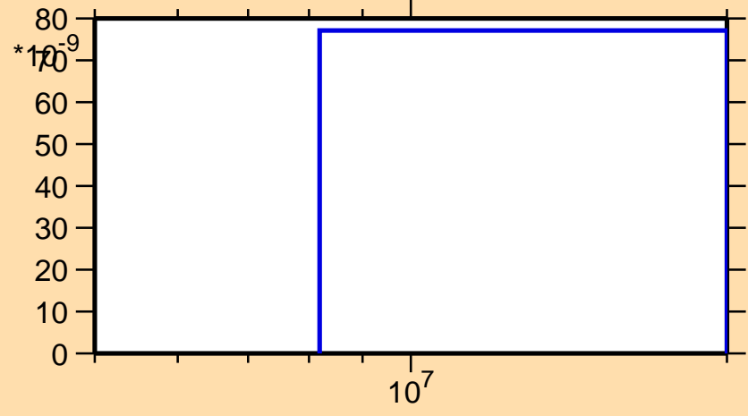
\sigma vs. E for ^{93}\text{Rh}(n,2np)
