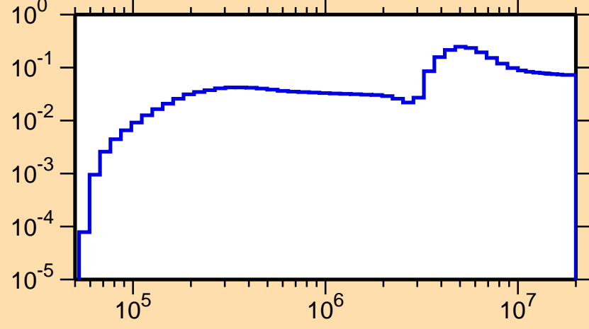
\sigma vs. E for ^{94}\text{Rh}(n,\text{inel.})
