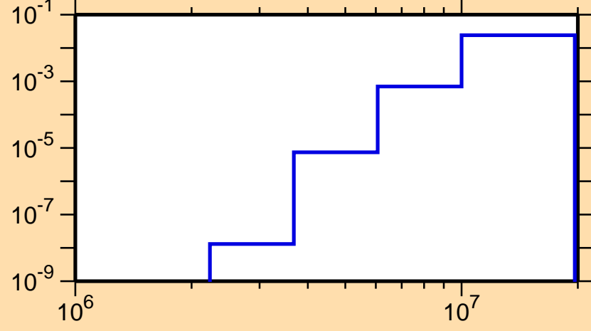
\sigma vs. E for ^{94}\text{Rh}(n,d)
