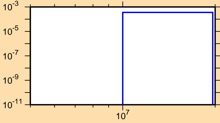
\sigma vs. E for ^{94}\text{Rh}(n,pd)
