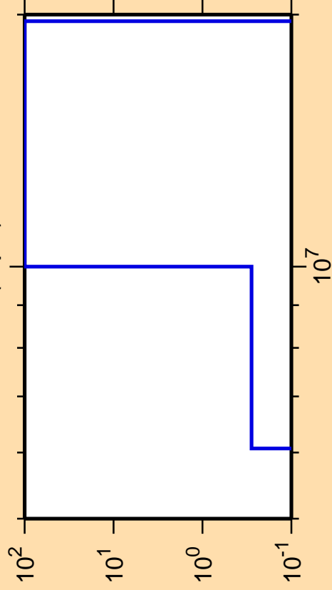
\Delta\sigma/\sigma vs. E for ^{94}\text{Rh}(n,pd)
