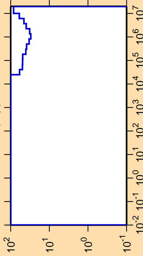
\Delta\sigma/\sigma vs. E for ^{94}\text{Rh}(n,p)
