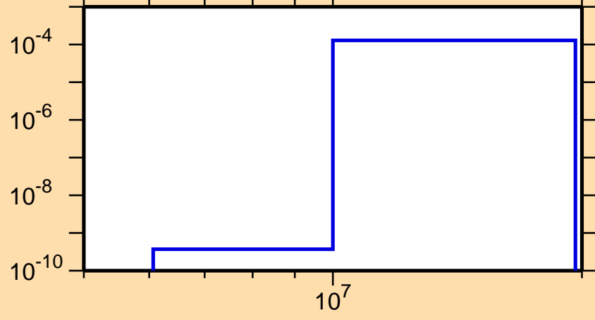
\sigma vs. E for ^{94}\text{Rh}(n,t)
