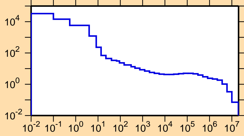
\sigma vs. E for ^{94}\text{Rh}(n,p)
