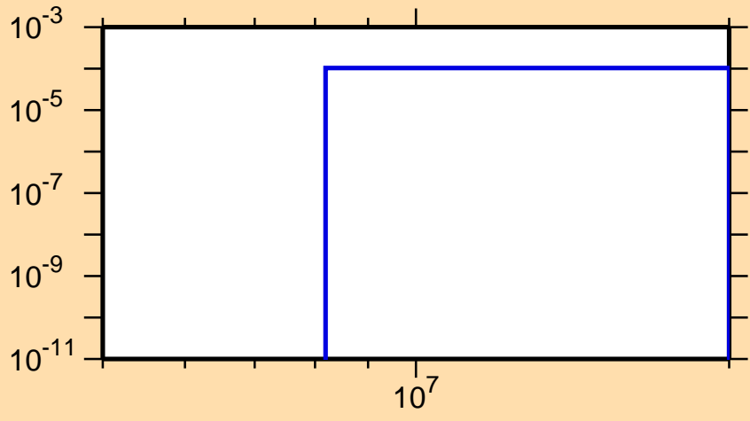
\sigma vs. E for ^{94}\text{Rh}(n,t)
