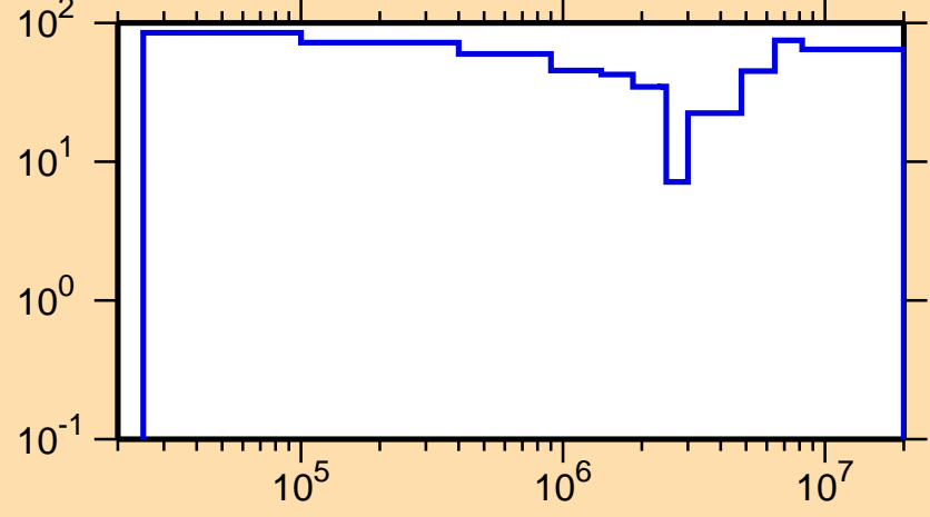
\Delta\sigma/\sigma vs. E for ^{94}\text{Rh}(n,n_1)
