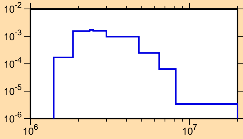
\sigma vs. E for ^{94}\text{Rh}(n,n_4)
