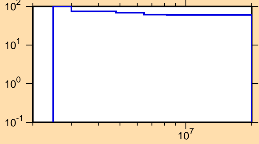
\Delta\sigma/\sigma vs. E for ^{94}\text{Rh}(n,n\text{cont.})
