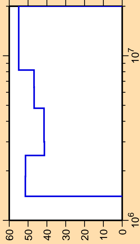
\Delta\sigma/\sigma vs. E for ^{94}\text{Rh}(n,n_4)
