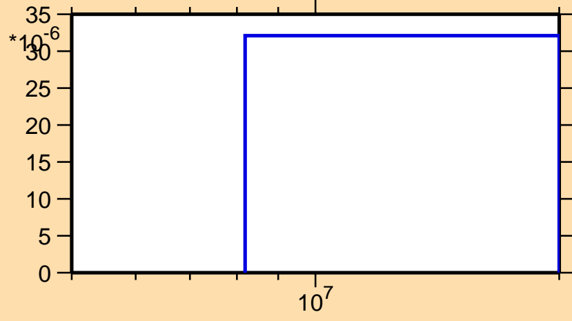
\sigma vs. E for ^{94}\text{Rh}(n,\alpha)
