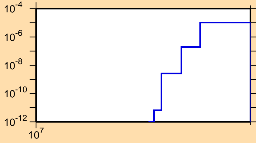
\sigma vs. E for ^{94}\text{Rh}(n,\text{pt})
