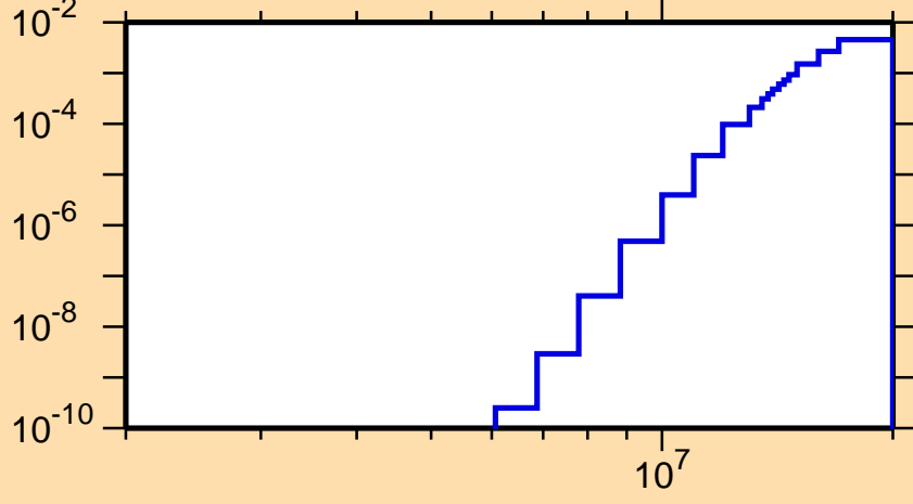
\sigma vs. E for ^{94}\text{Rh}(n,\text{He3})
