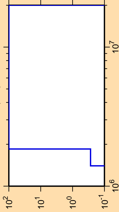
\Delta\sigma/\sigma vs. E for ^{94}\text{Rh}(n,d)
