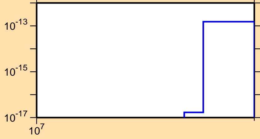
\sigma vs. E for ^{95}\text{Rh} (mt 34)
