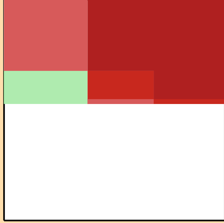
\Delta\sigma/\sigma vs. E for ^{95}\text{Rh}(n,\text{el.})
