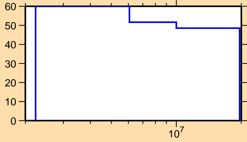
\Delta\sigma/\sigma vs. E for ^{95}\text{Rh}(n,ncont.)
