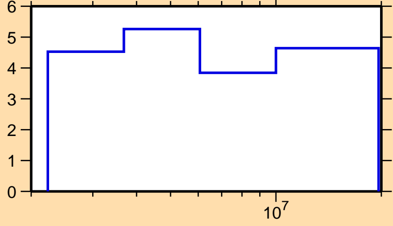
\Delta\sigma/\sigma vs. E for ^{95}\text{Rh}(n,\text{nonel.})
