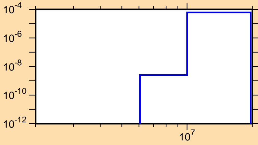
\sigma vs. E for ^{95}\text{Rh}(n,\text{He3})
