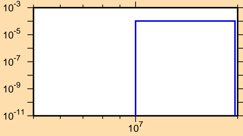
\sigma vs. E for ^{95}\text{Rh}(n,\text{pd})
