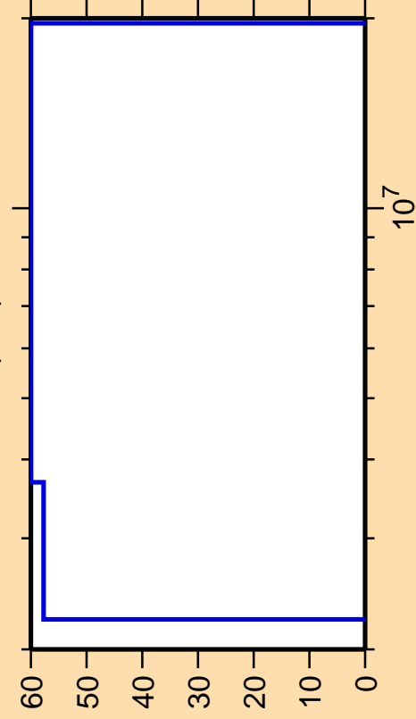
\Delta\sigma/\sigma vs. E for ^{95}\text{Rh}(n,d)
