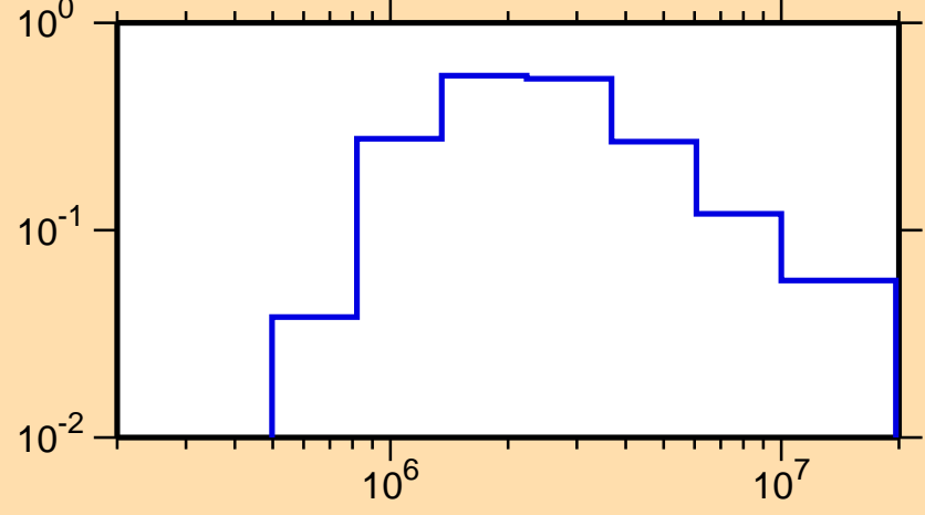
\sigma vs. E for ^{95}\text{Rh}(n,\text{inel.})
