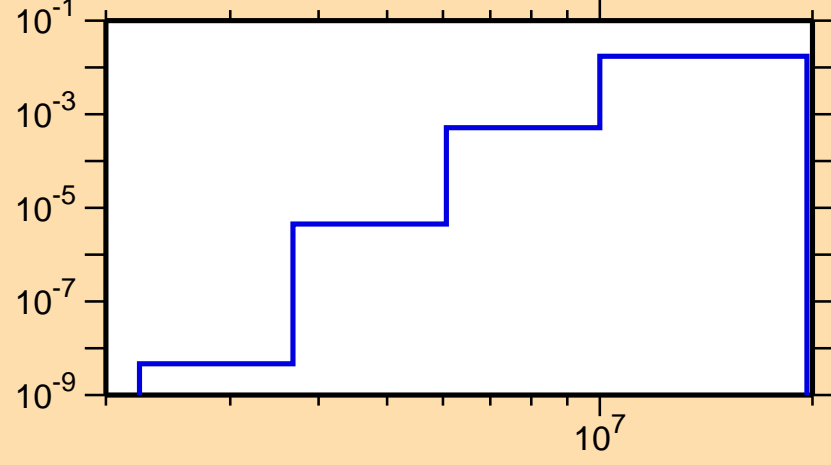
\sigma vs. E for ^{95}\text{Rh}(n,d)
