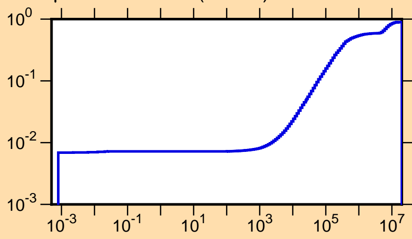
\mu vs. E for ^{98}\text{Rh}(\text{mt251})
