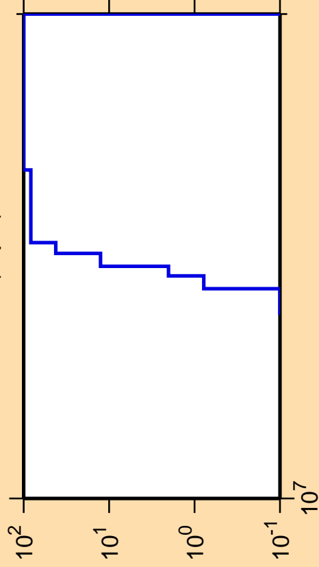
\Delta\sigma/\sigma vs. E for ^{98}\text{Rh}(n,pd)
