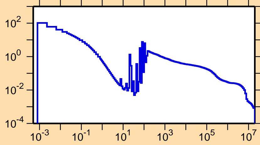
\sigma vs. E for ^{98}\text{Rh}(n,\gamma)
