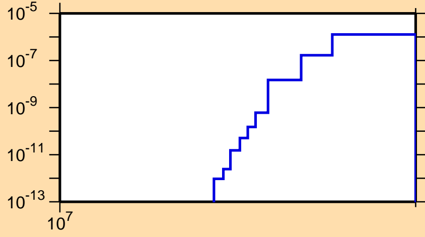
\sigma vs. E for ^{98}\text{Rh}(n,pd)
