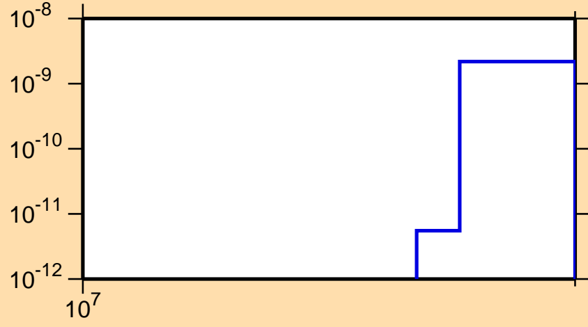
\sigma vs. E for ^{98}\text{Rh} (mt 34)
