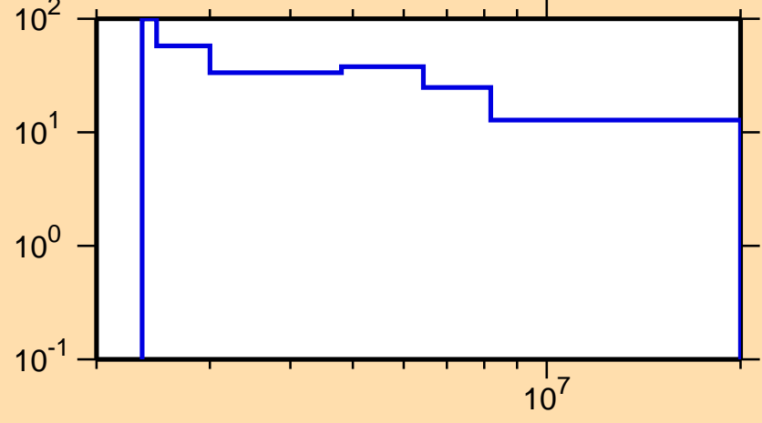
\Delta\sigma/\sigma vs. E for ^{98}\text{Rh}(n,n\text{cont.})
