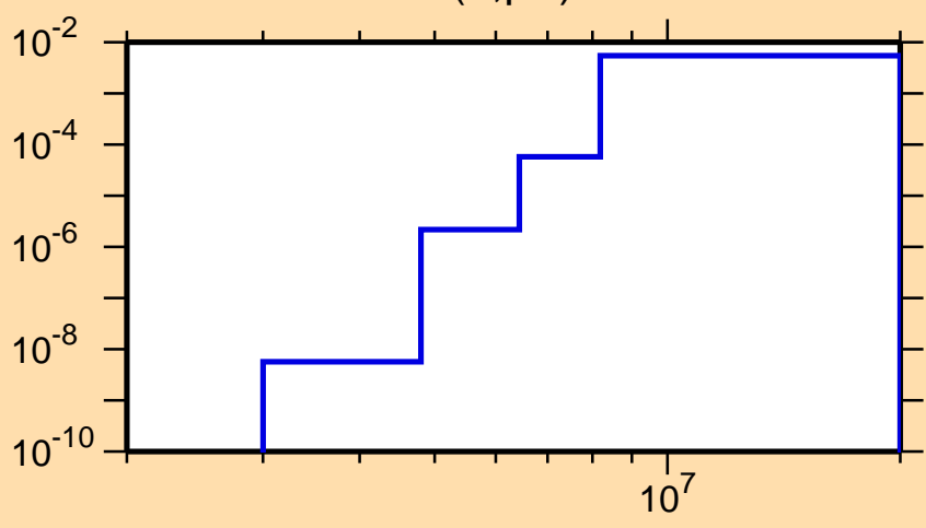
\sigma vs. E for ^{98}\text{Rh}(n,p\alpha)
