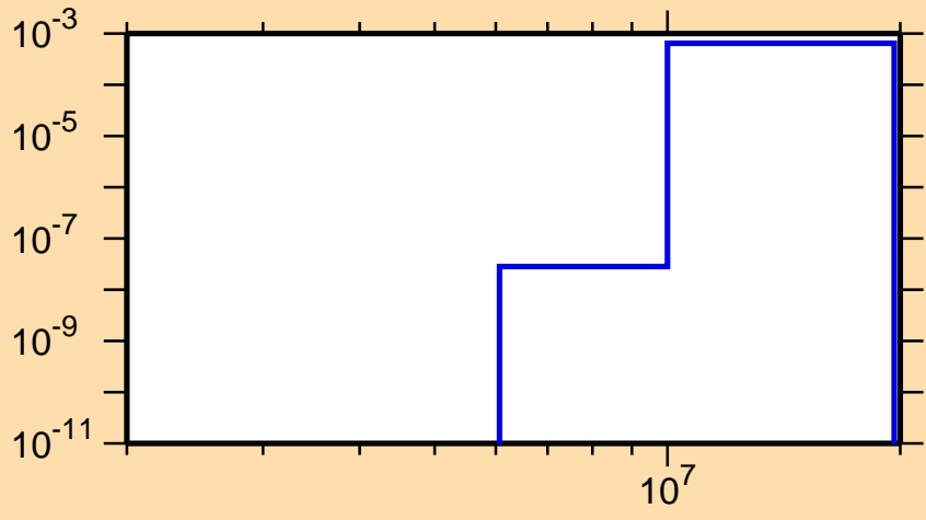
\sigma vs. E for ^{98}\text{Rh}(n,t)
