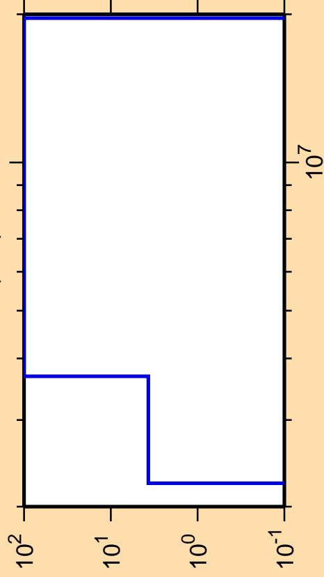
\Delta\sigma/\sigma vs. E for ^{98}\text{Rh}(n,d)
