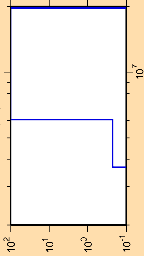
\Delta\sigma/\sigma vs. E for ^{98}\text{Rh}(n,t)
