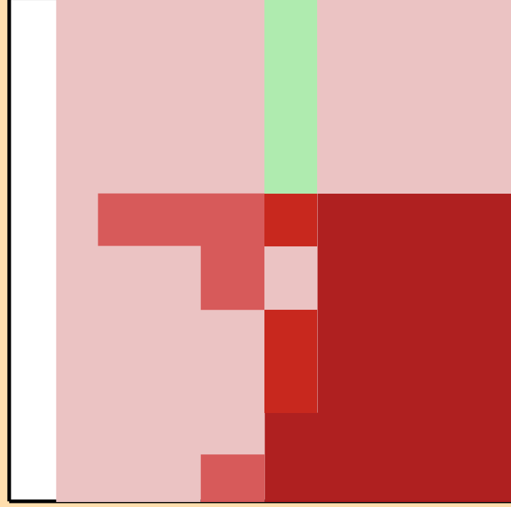
\Delta\sigma/\sigma vs. E for ^{98}\text{Rh}(n,n\text{cont.})
