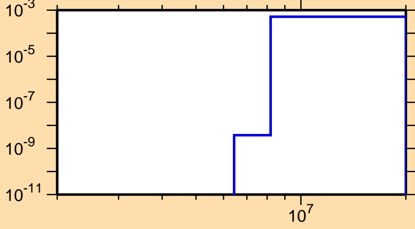
\sigma vs. E for ^{98}\text{Rh}(n,t)
