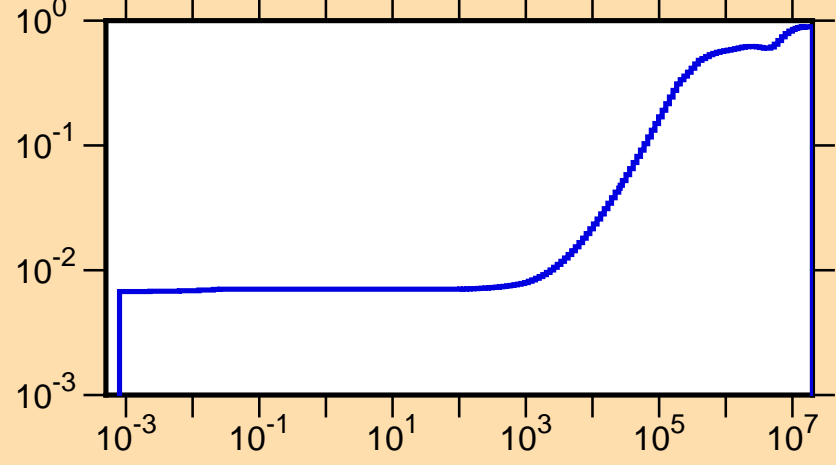
\mu vs. E for ^{100}\text{Rh}(\text{mt251})
