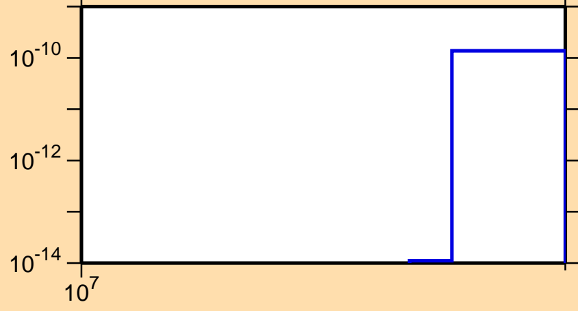
\sigma vs. E for ^{100}\text{Rh}(n,\text{pt})
