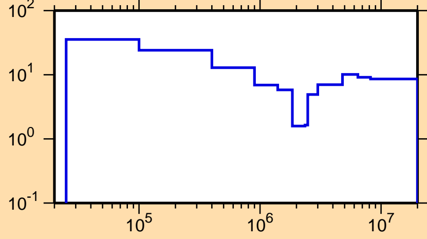
\Delta\sigma/\sigma vs. E for ^{100}\text{Rh}(n,\text{nonel.})
